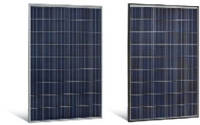
AX P-54 3.2 premium polycrystalline Rated power 230/235/240 Wp 40 mm aluminium frame silver or black Backsheet white or black
